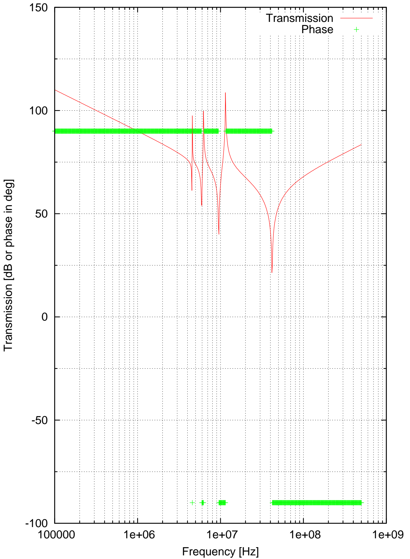
Transmission of PIN diode reactor
