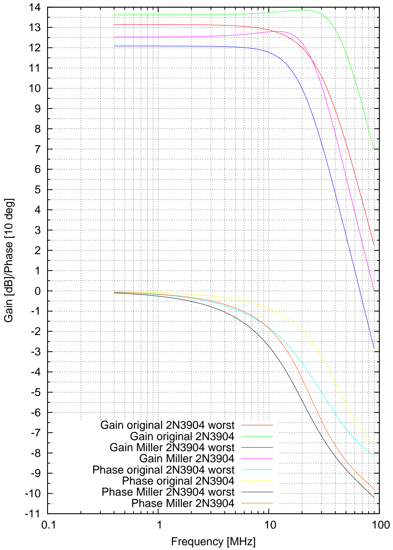
Bandwidth sensitivity to Miller effect
