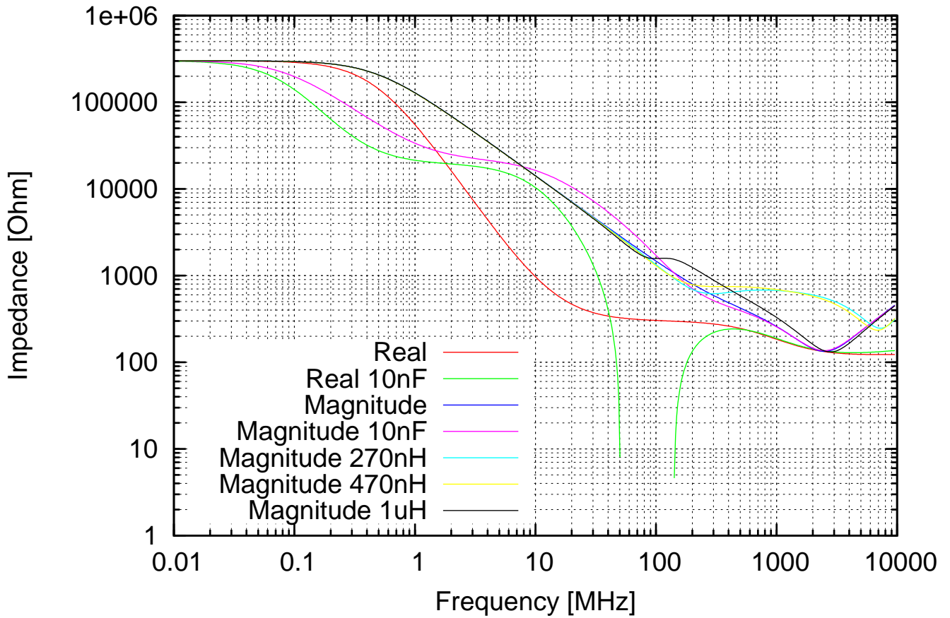
Current Source Output Impedance
