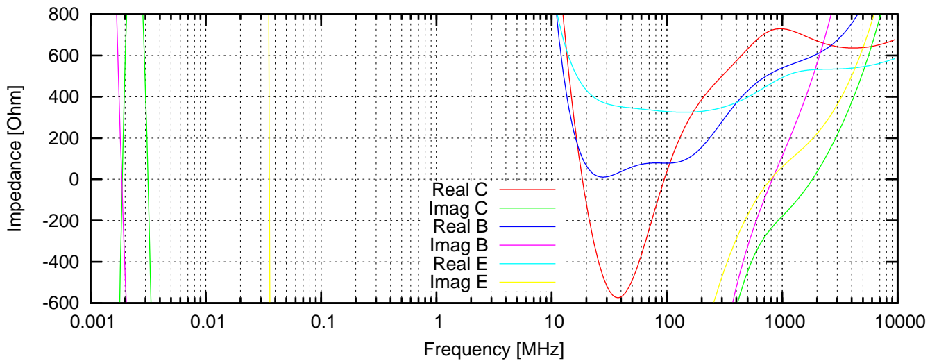
On Transistor With Resonator 50 MHz 2pF 5uH 600 Ohm
