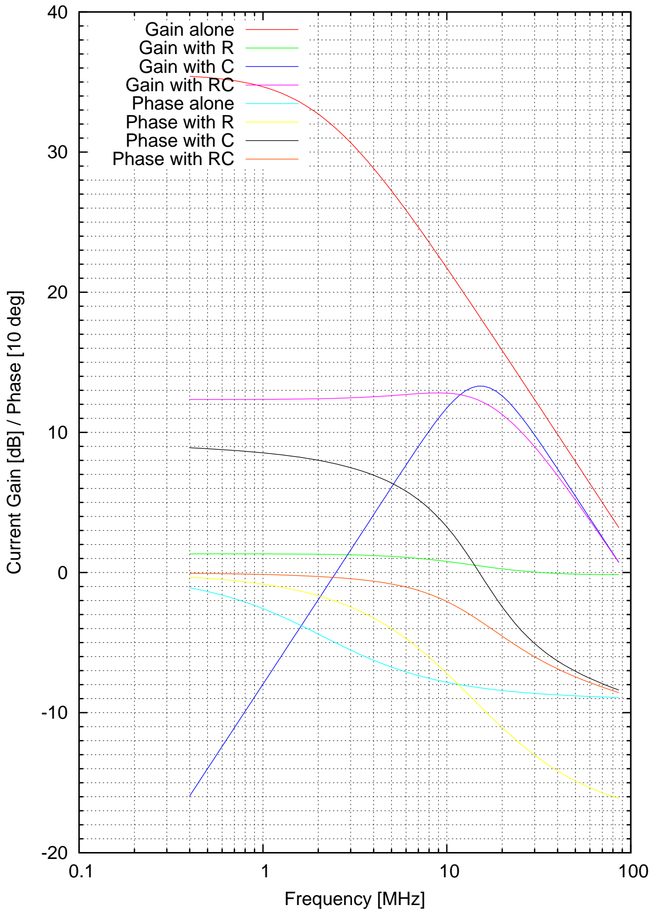
Basic 2N3904 Long Tail Pair Frequency Response Of Current Gain
