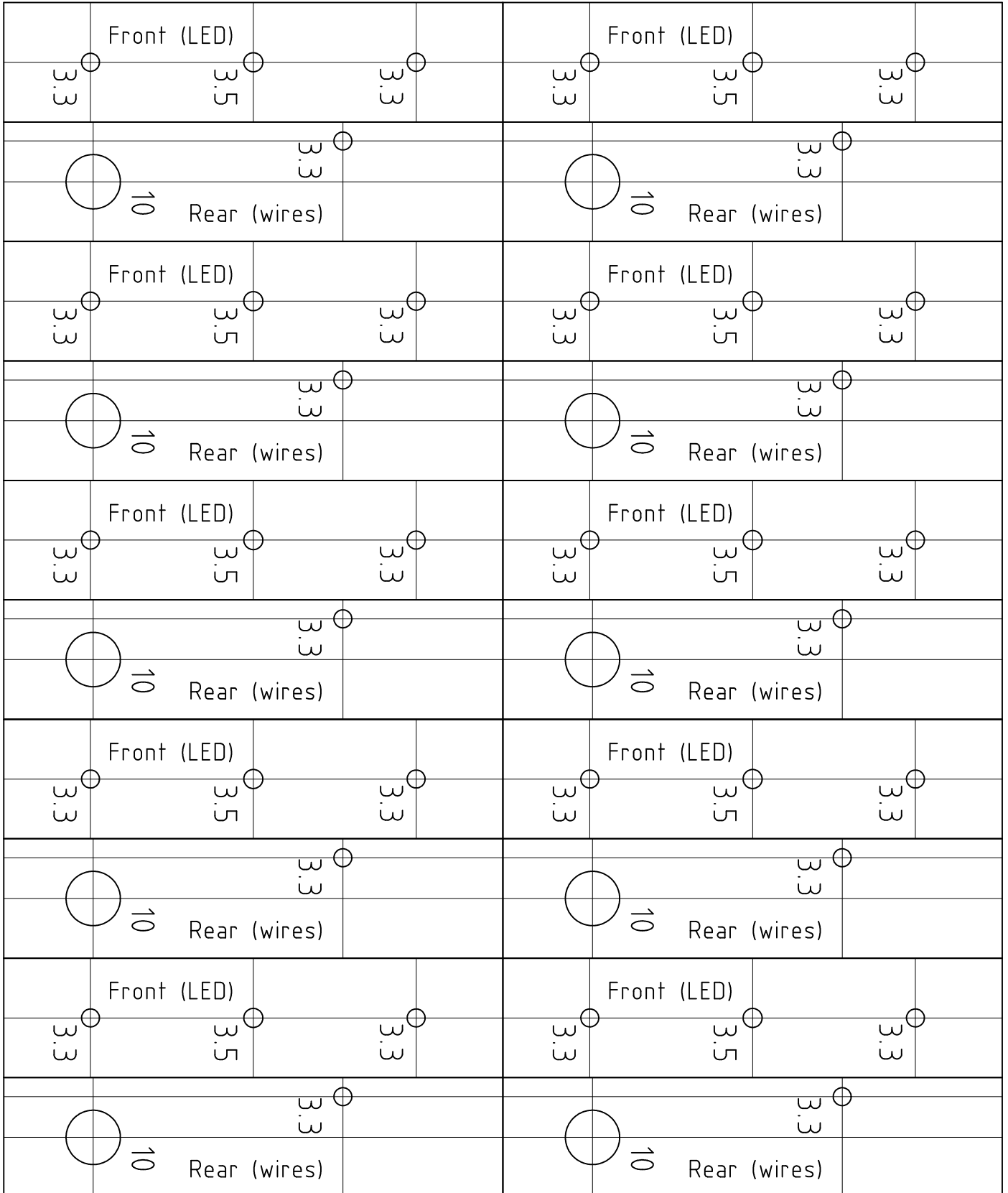
PCB Transmitter template for 10 boxes
