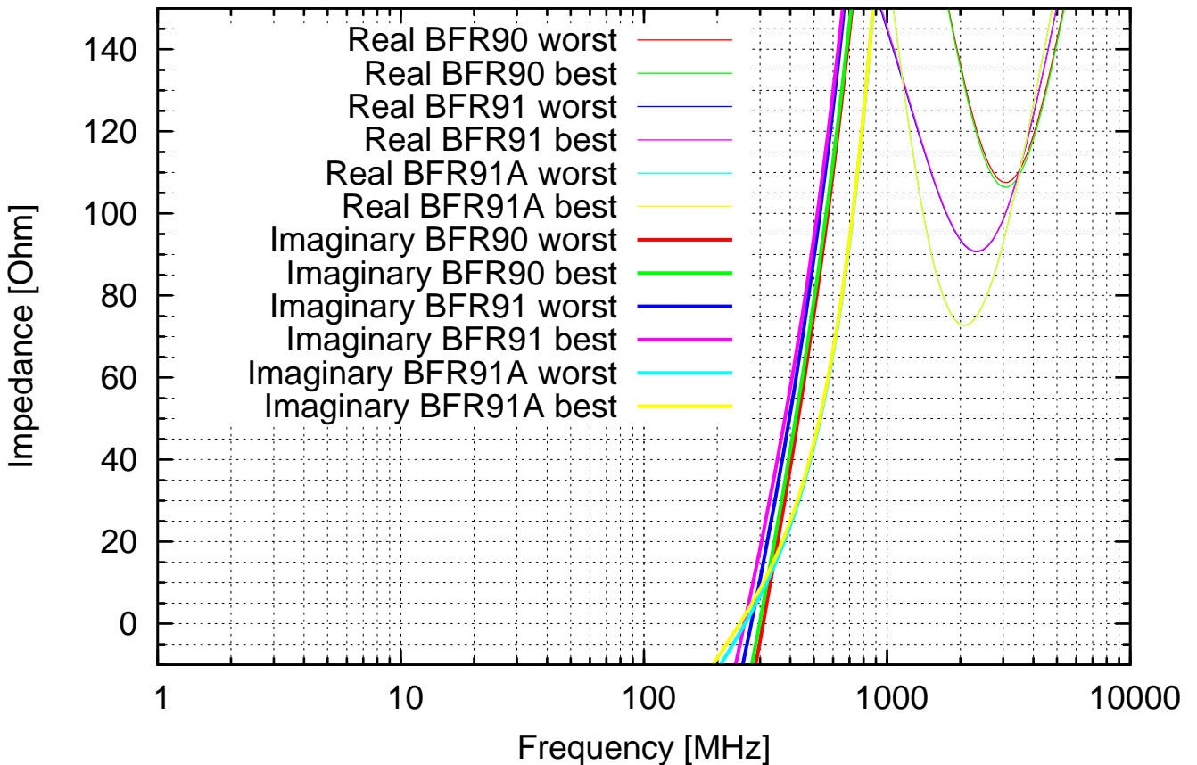
BFR90, BFR91, and BFR91A Interstage Impedance
