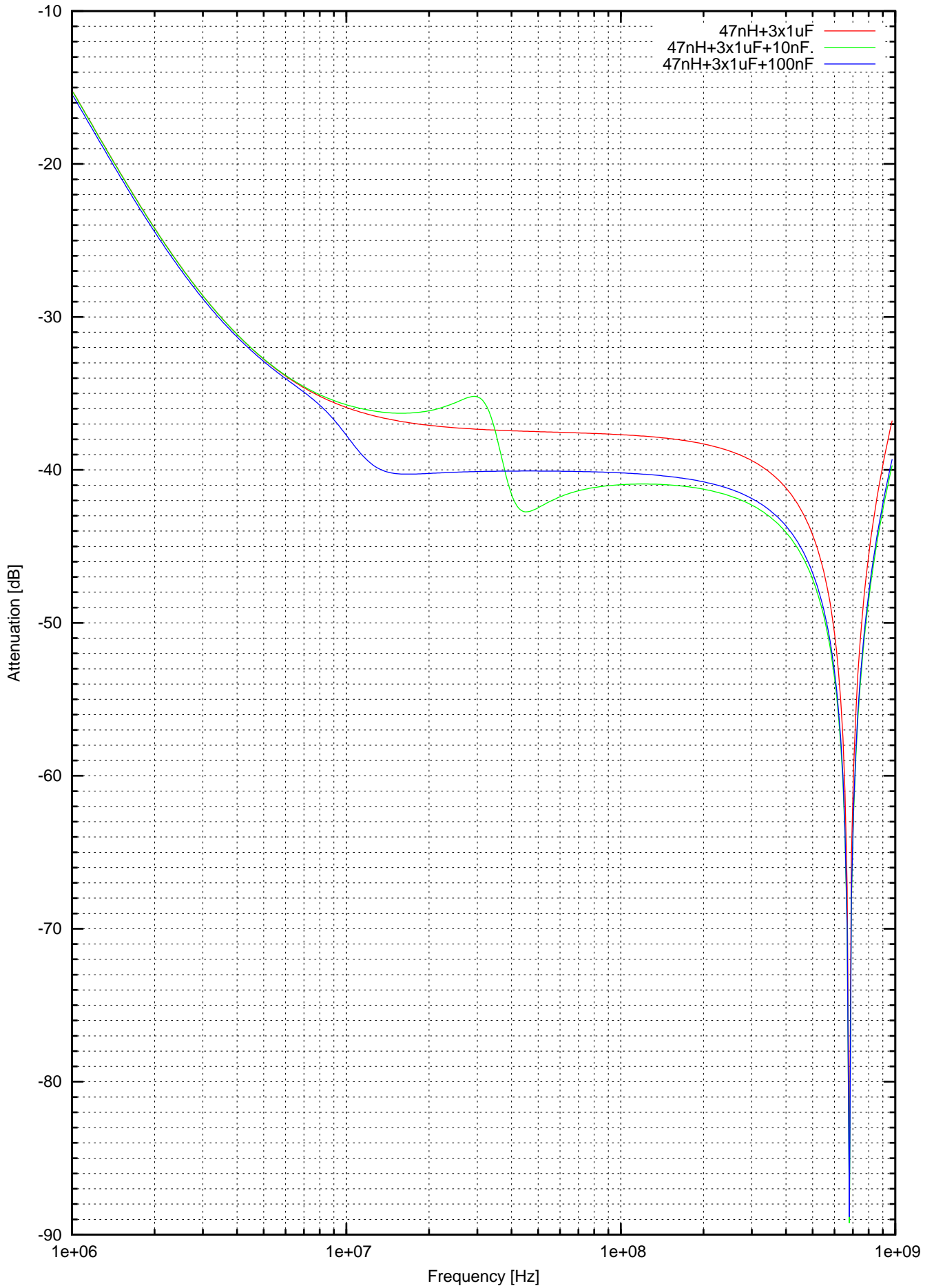
Attenuation of shielding filter
