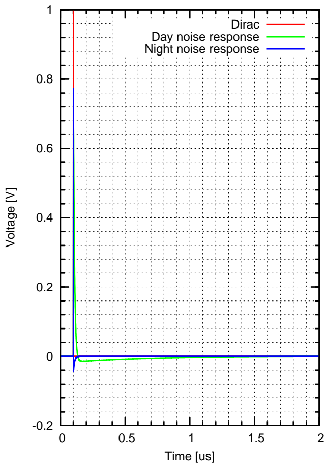
Impulse Response of Ronja 10M Receiver
