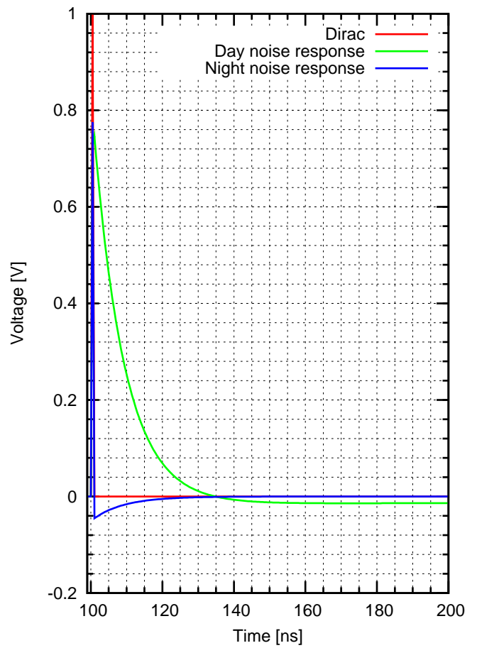
Impulse Response of Ronja 10M Receiver
