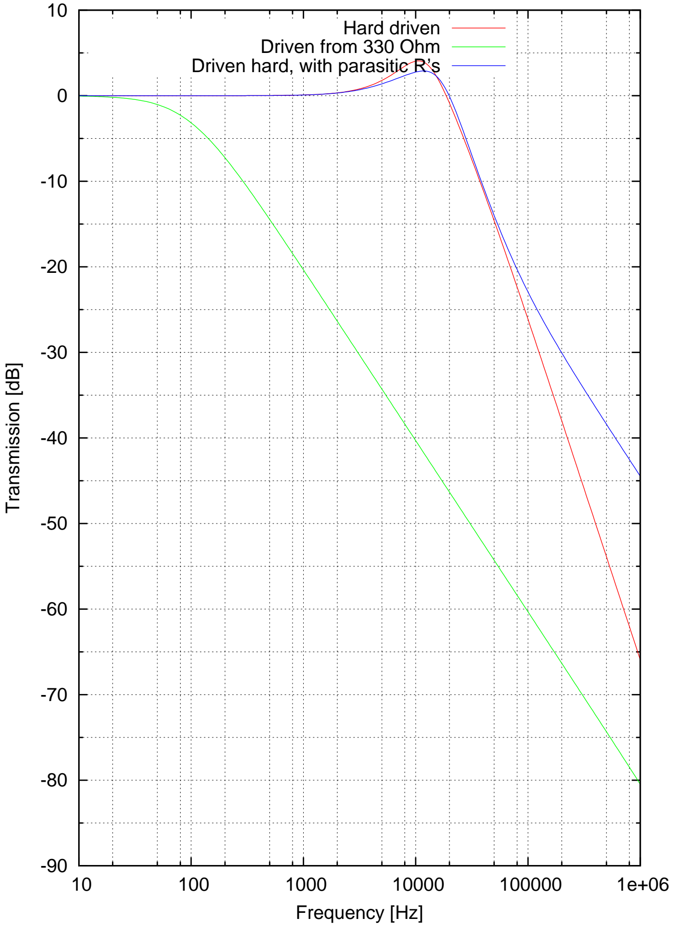
Transmission of RX power filter
