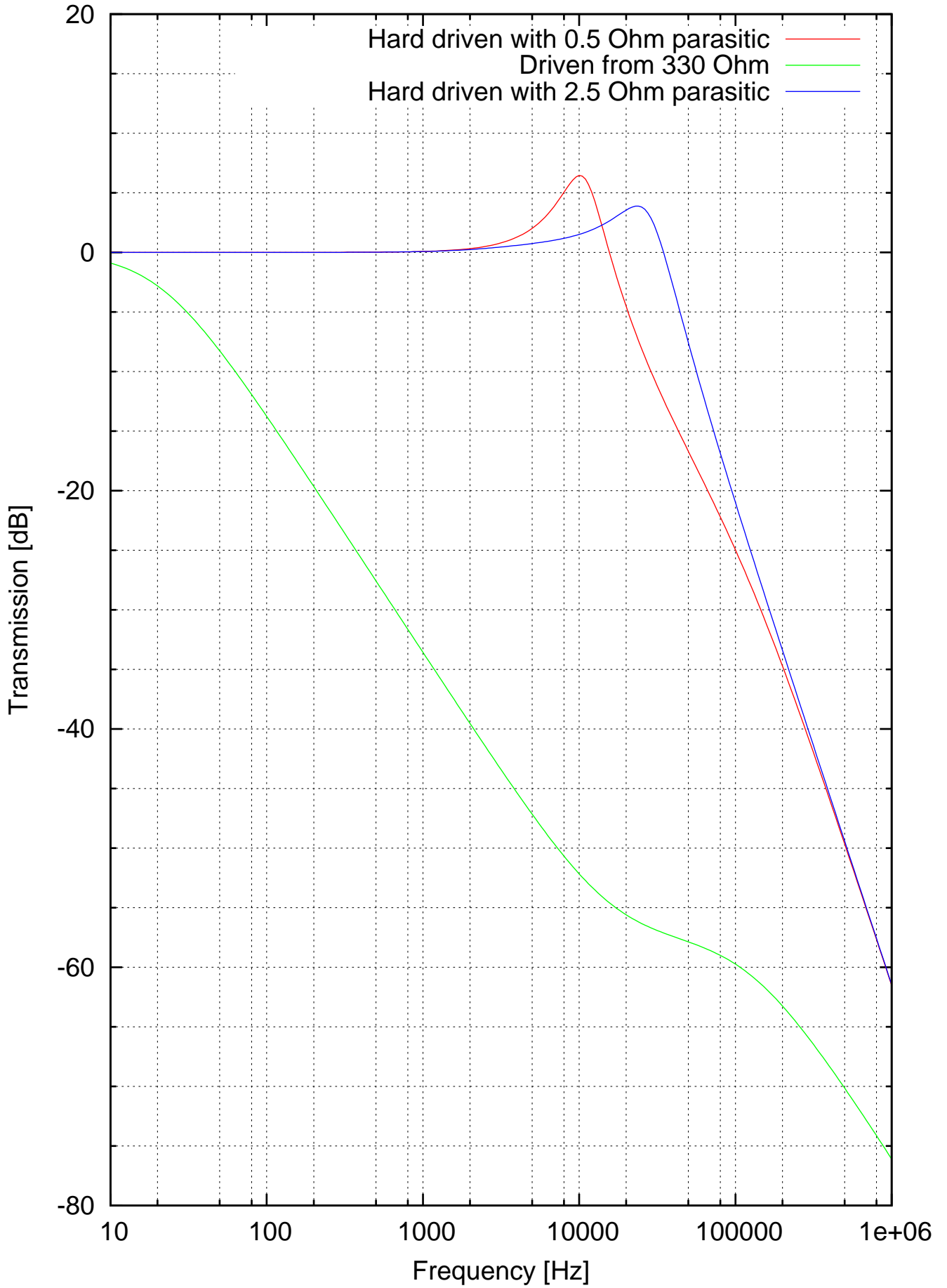
Transmission of 3rd RX power filter
