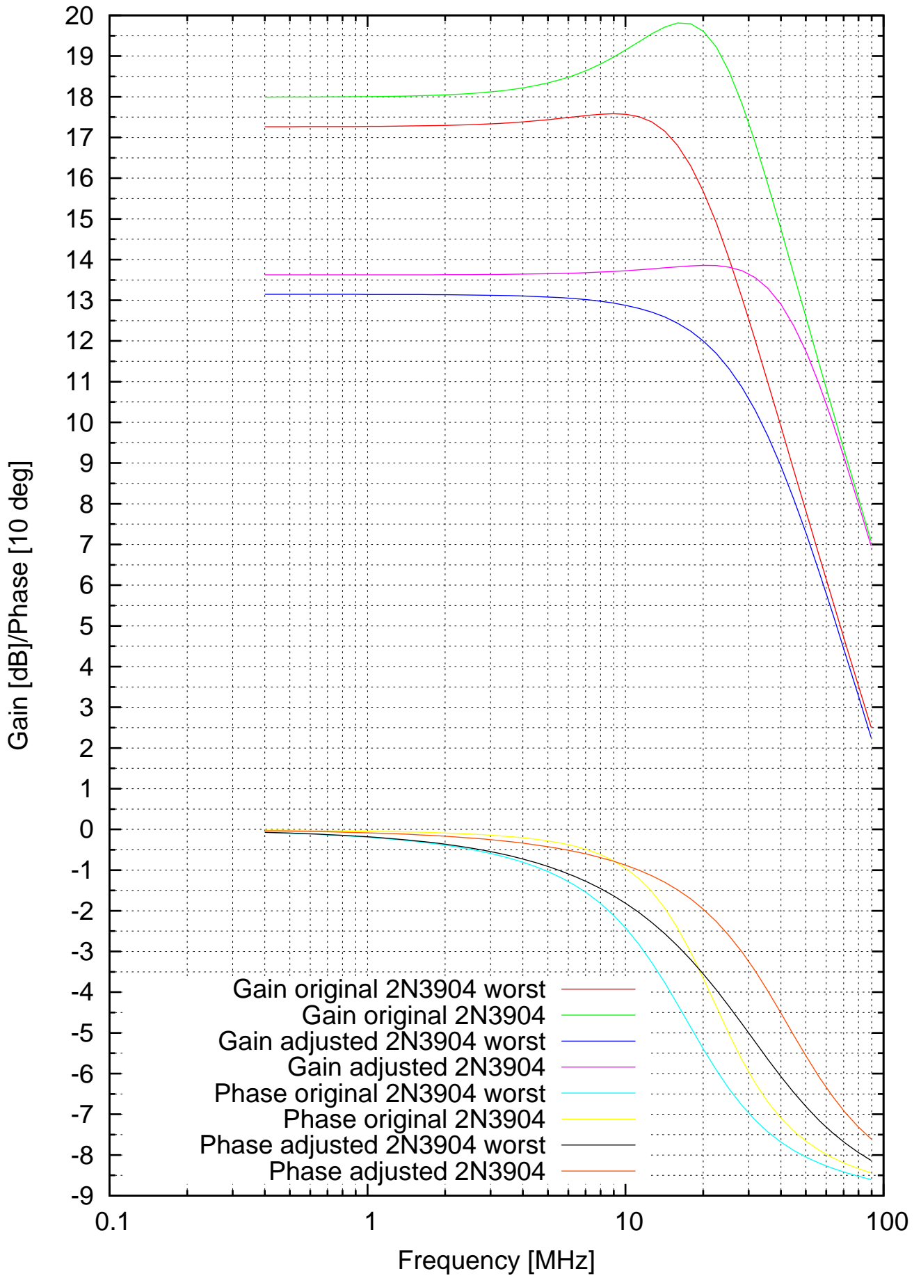
Bandwidth sensitivity to transistor parameters
