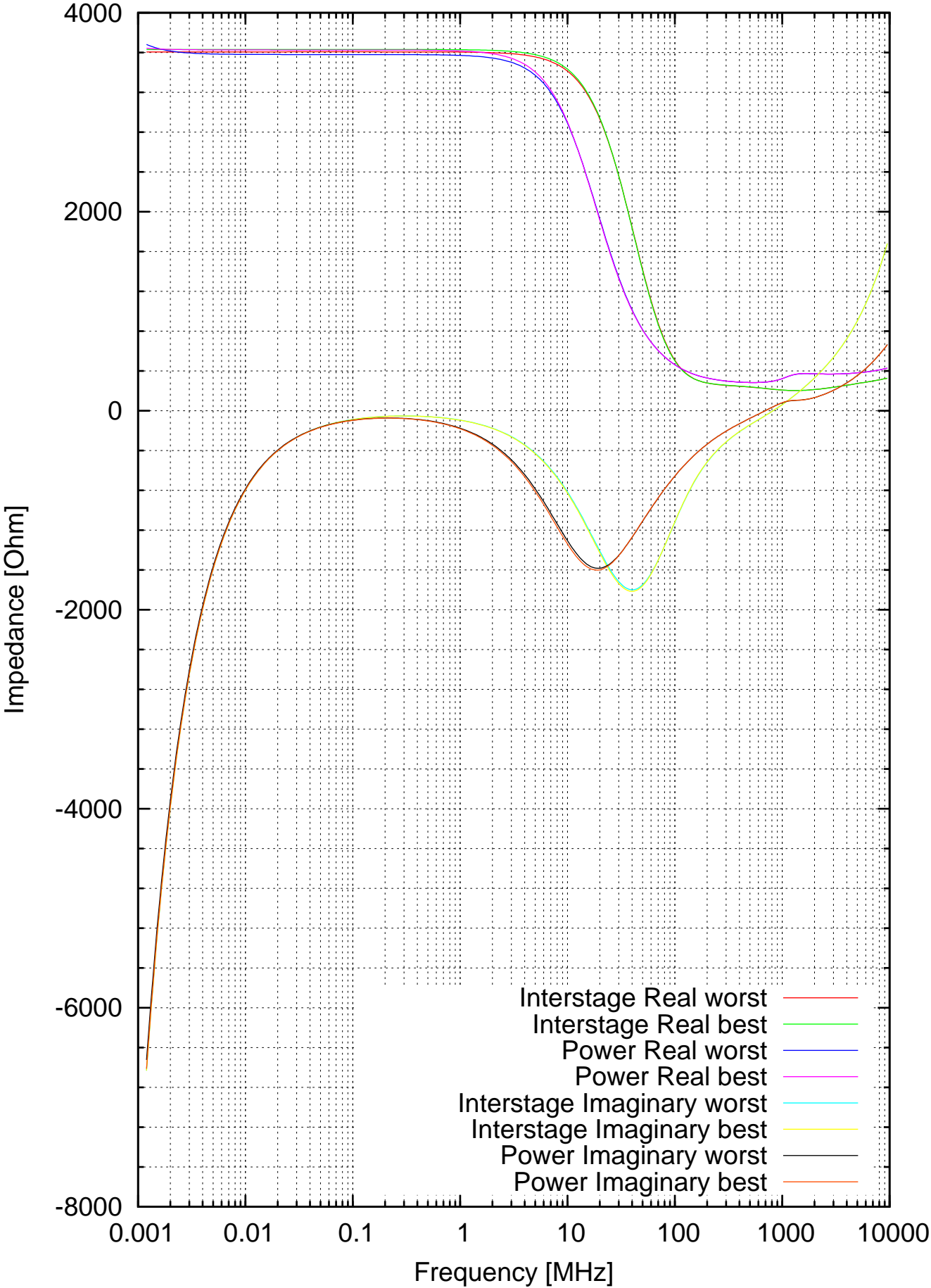
BFR91A longitudinal stability
