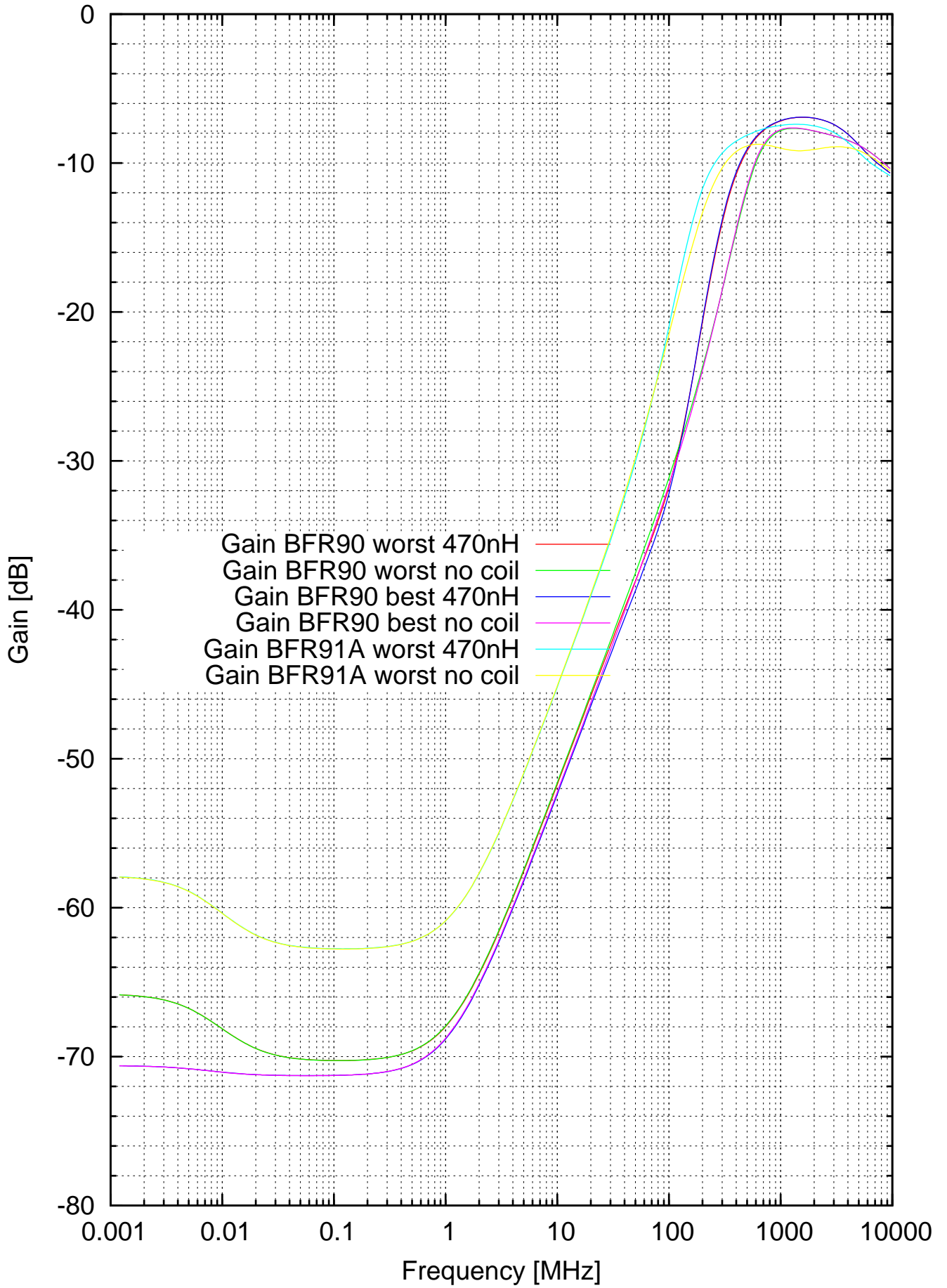
BFR90 and 91A longitudinal mode gain
