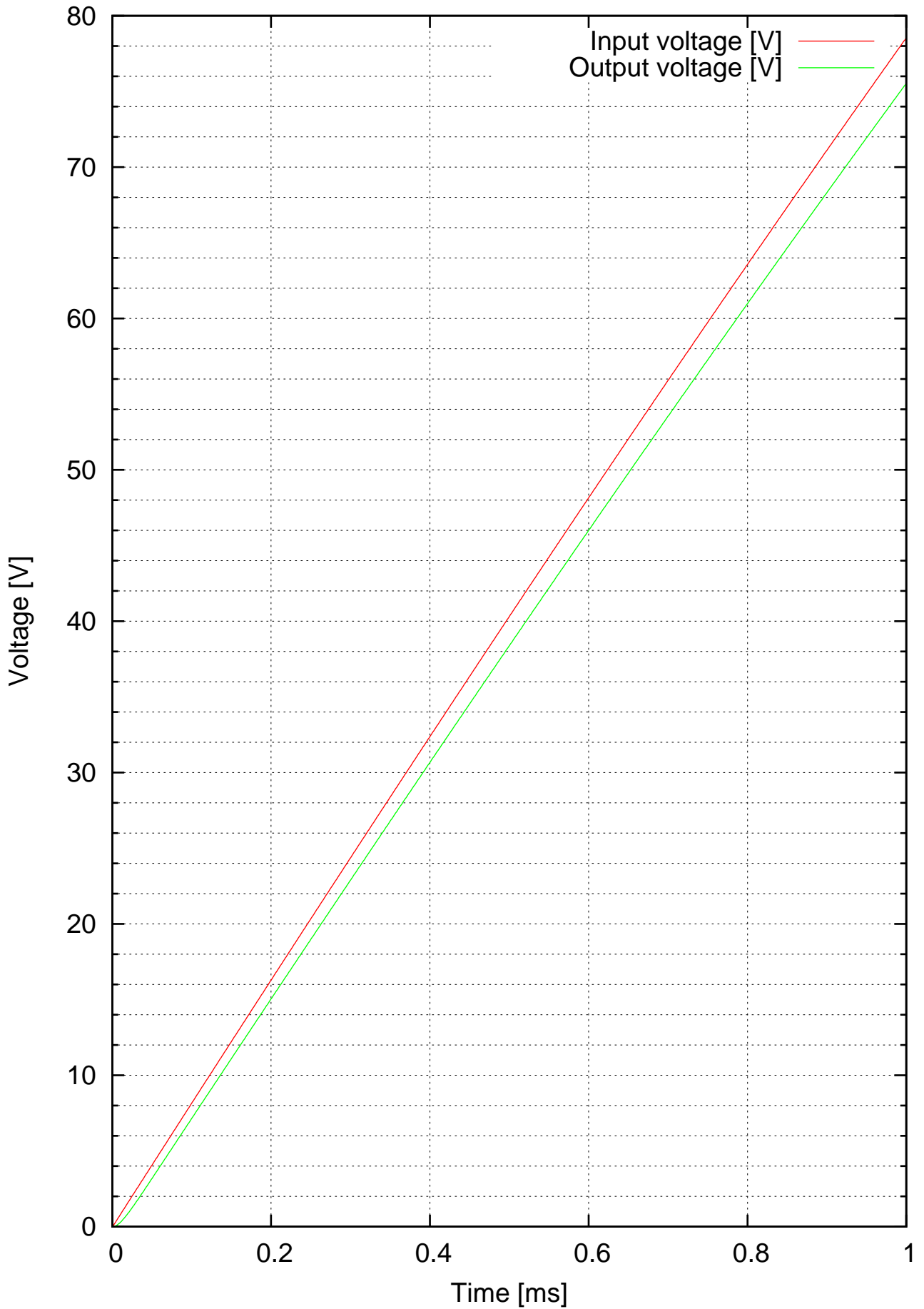
Transient response of Exciter when 0.5A of load is removed
