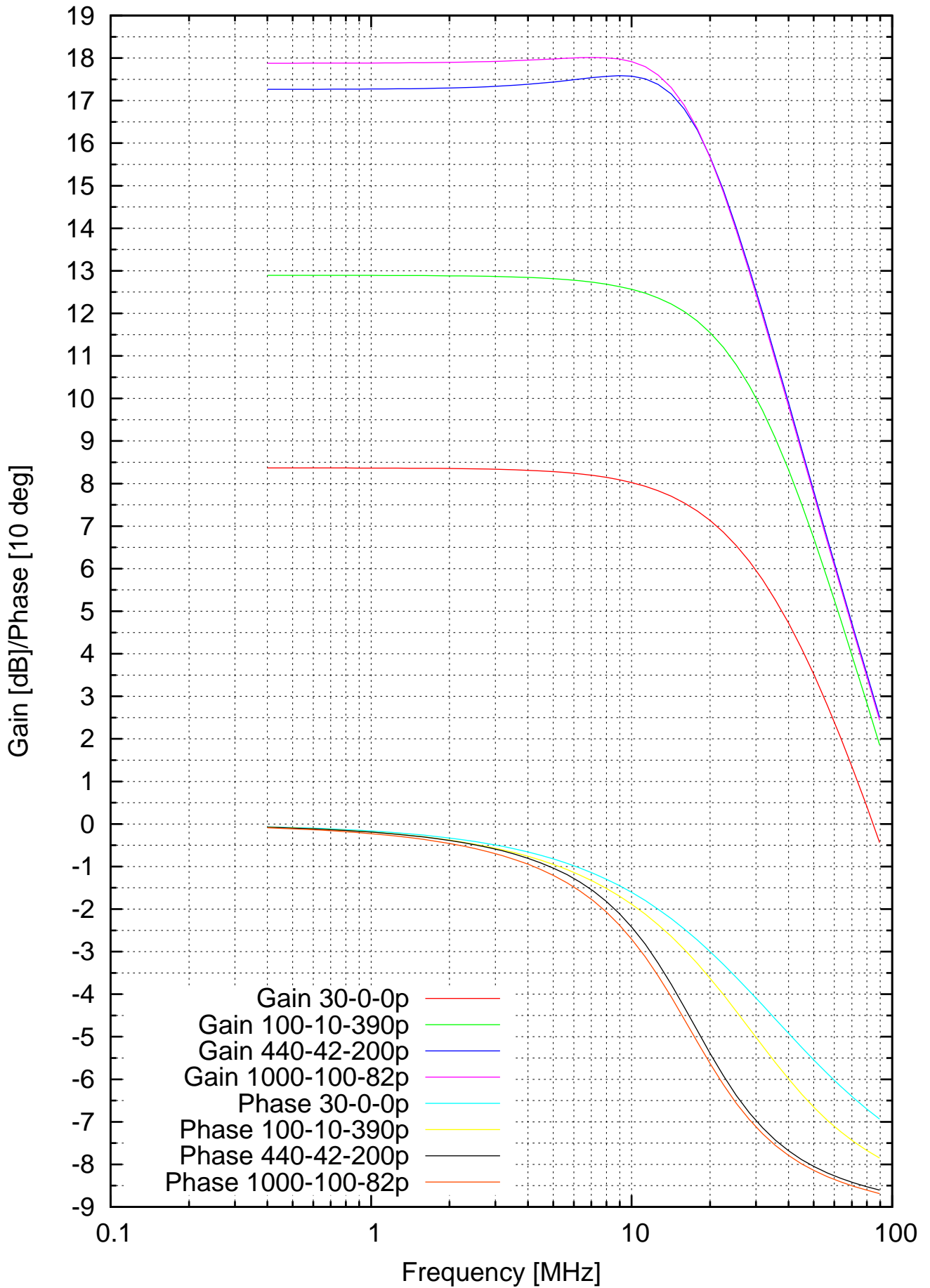
Worst Case (fT, beta) 2N3904 Pimped Amplifier Frequency Response
