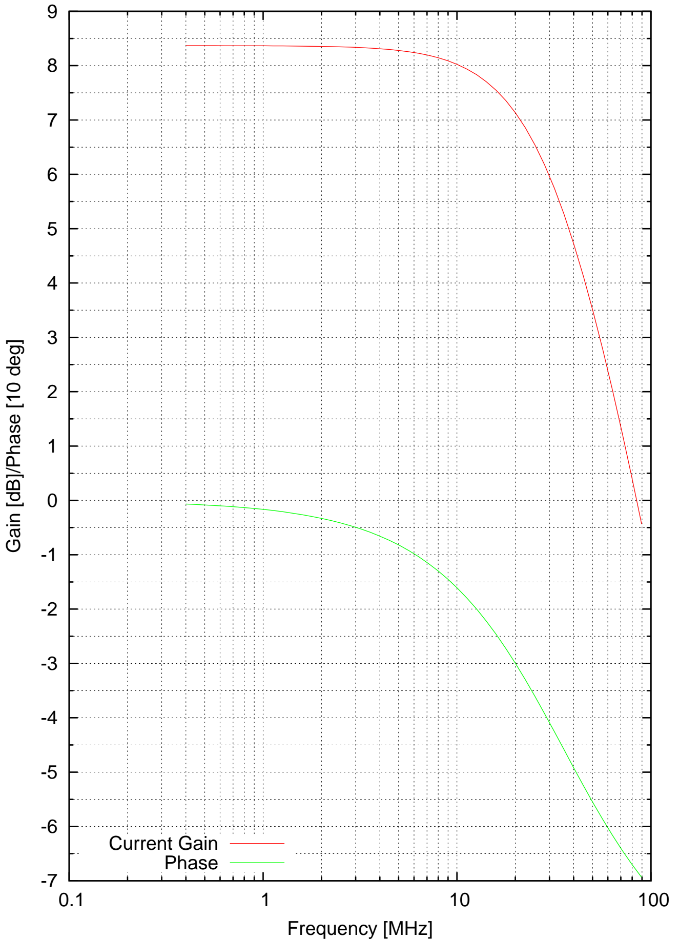
Worst Case (fT, beta) 2N3904 Amplifier Frequency Response
