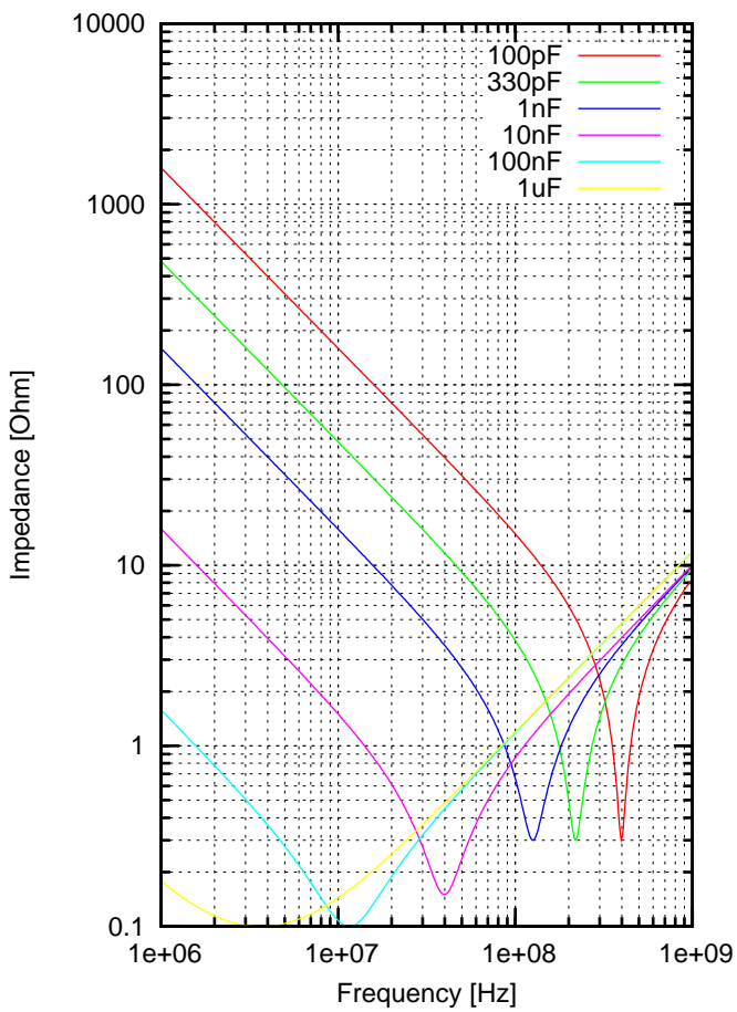
Impedance of 100pF-1uF ceramic capacitors
