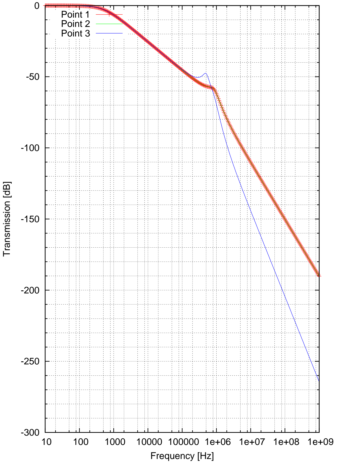
Transmission of RX base bus filters
