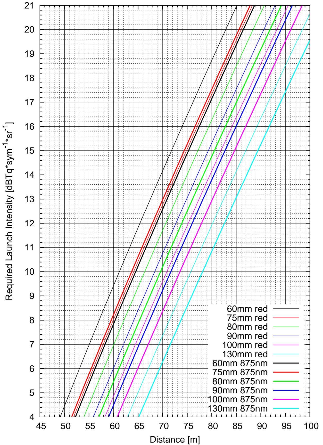
Required LED flux vs. distance (50m visibility = 340 dB/km)
