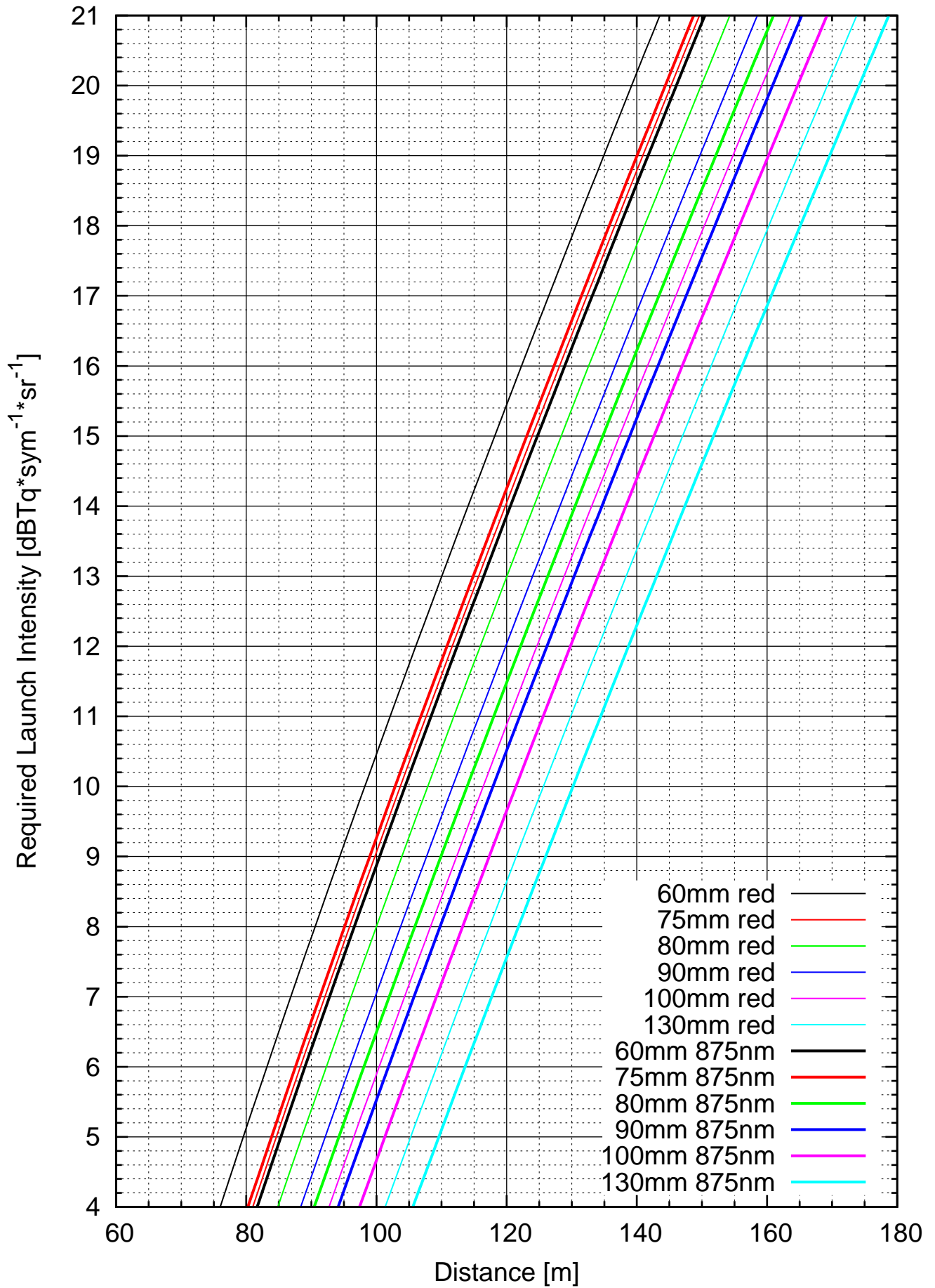
Required LED flux vs. distance (100m visibility = 170 dB/km)
