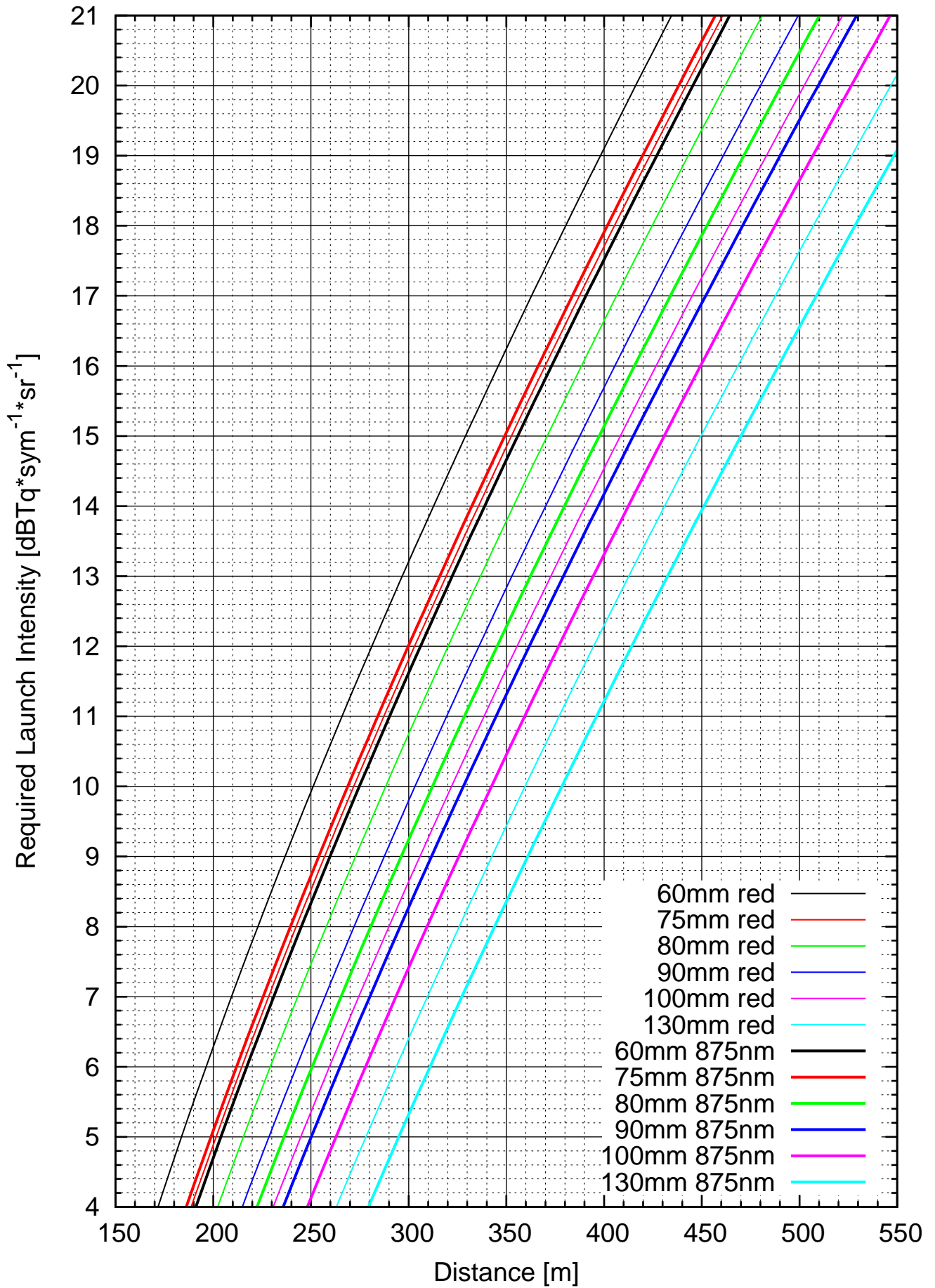
Required LED flux vs. distance (500m visibility = 34 dB/km)
