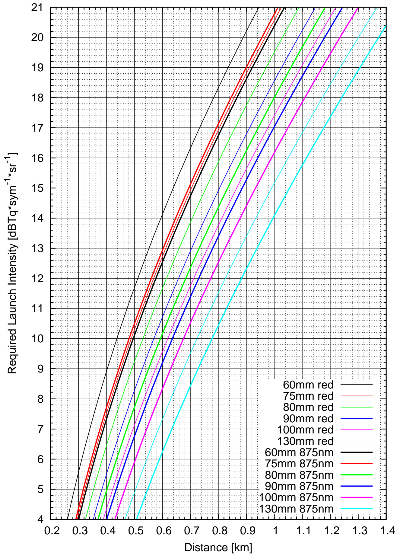
Required LED flux vs. distance (2km visibility = 8.5 dB/km)
