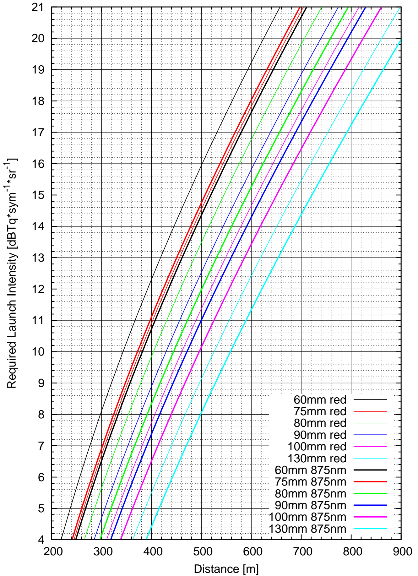
Required LED flux vs. distance (1km visibility = 17 dB/km)
