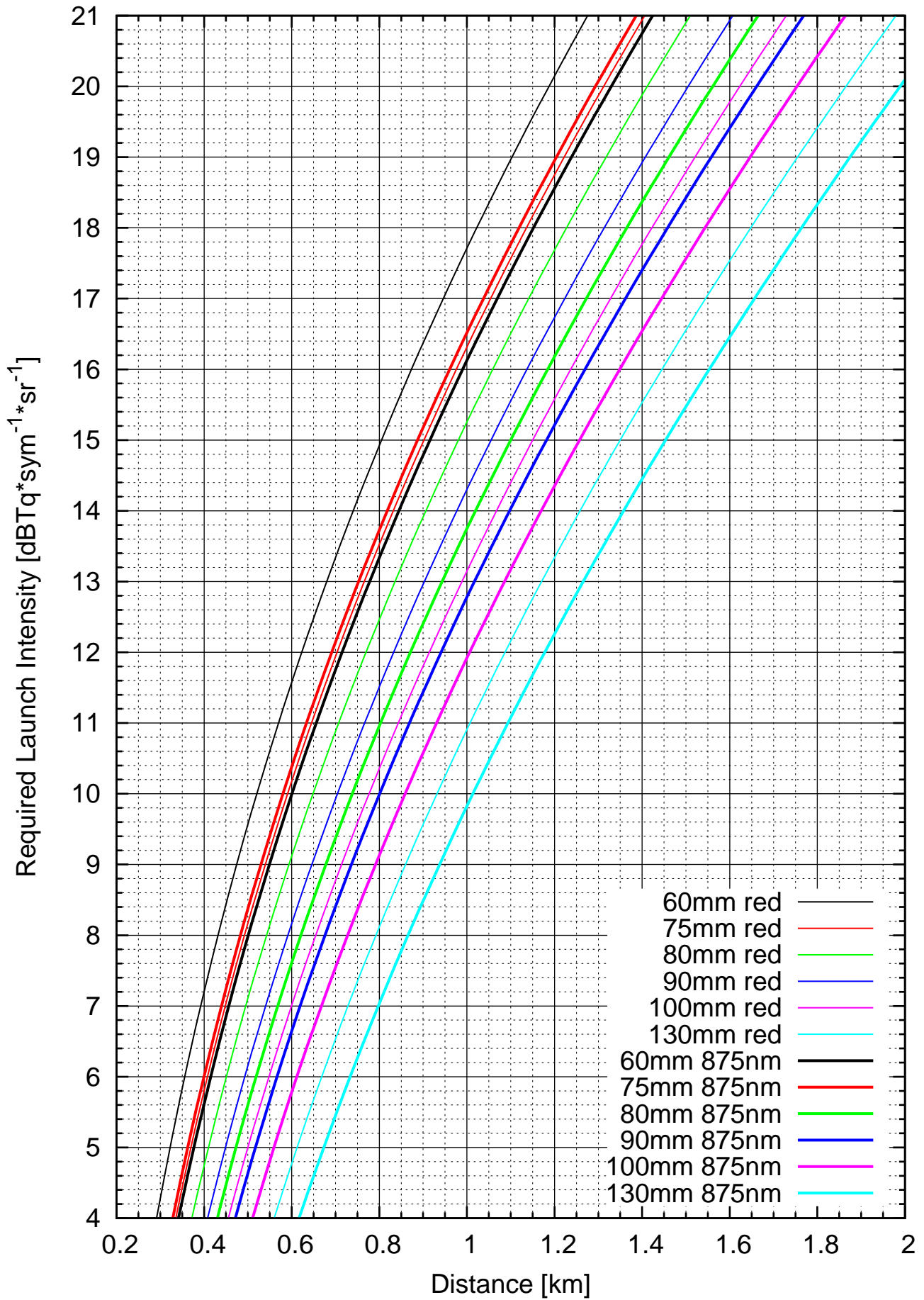
Required launch intensity vs. distance (4km visibility = 4.25 dB/km)
