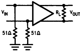
Test Circuit 1
