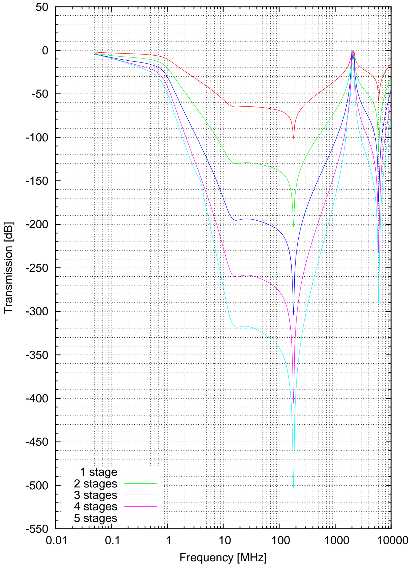
Transmission of Mundaka LNA 2-fold power filter
