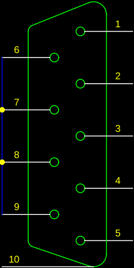
DE-9 female
